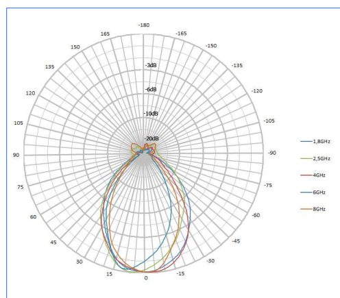
Horizontal Pattern HyperLOG 3080 X
