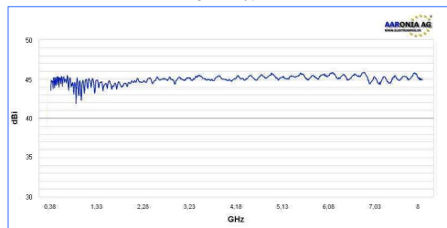
Gain Diagram HyperLOG 30100X
