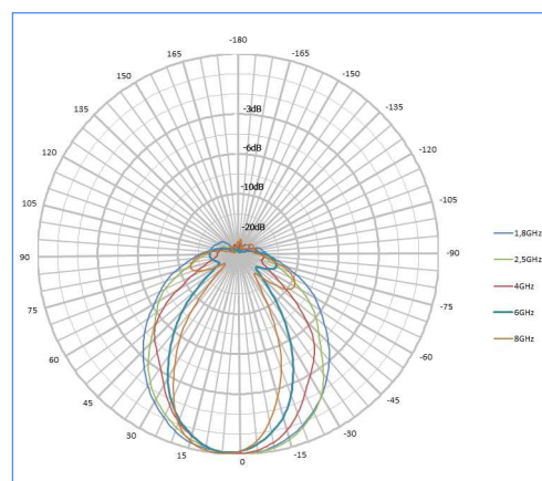
Vertikal Pattern HyperLOG 3080 X
